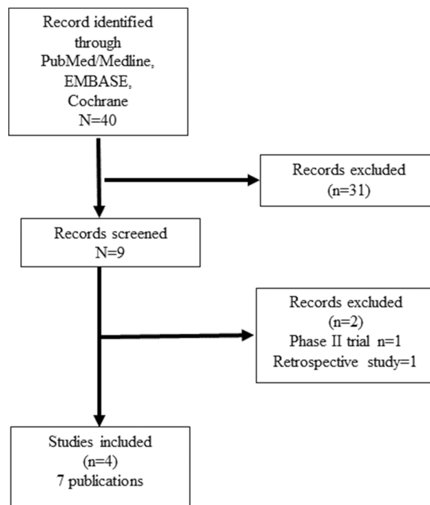
Figure 1 PRISMA diagram of clinical trials of ruxolitinib in polycythemia vera.
