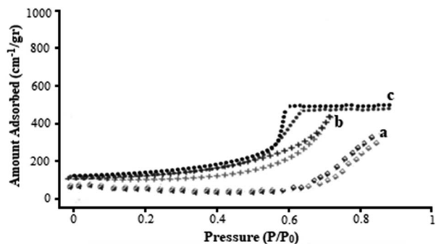
Fig. 6 N_2 adsorption–desorption isotherms \beta -CDs (a), Ni-based MOF (b), and \beta -CDs/Ni-based MOF composite (c).
