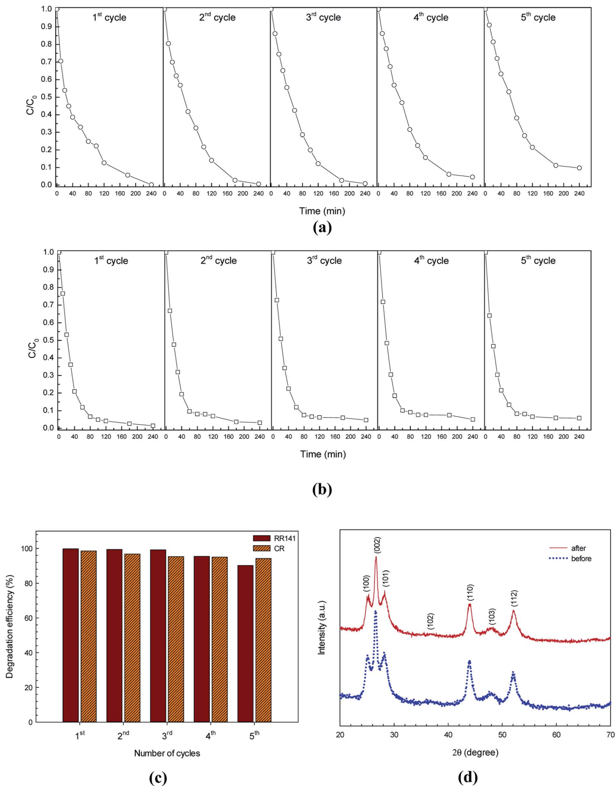
Fig. 10 Reusability of the CdS photocatalyst for photodegradation of RR141 azo dye (a) and CR dye (b) for five cycles under white light irradiation, bar chart of reusability of the CdS photocatalyst for both dyes (c) and XRD patterns of the CdS photocatalyst before and after photodegradation of azo dye (d).
