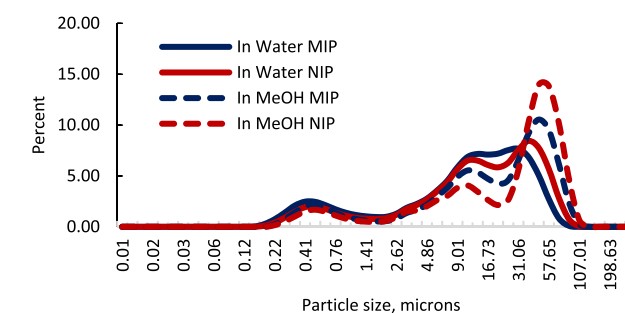
Figure 3. Hydrodynamic particle size distribution (%) molecularly imprinted (MIP, blue) and non-imprinted (red) polymers in water (solid line) and in 5% methanol (dotted line) by dynamic light scattering (DLS) measurements.
