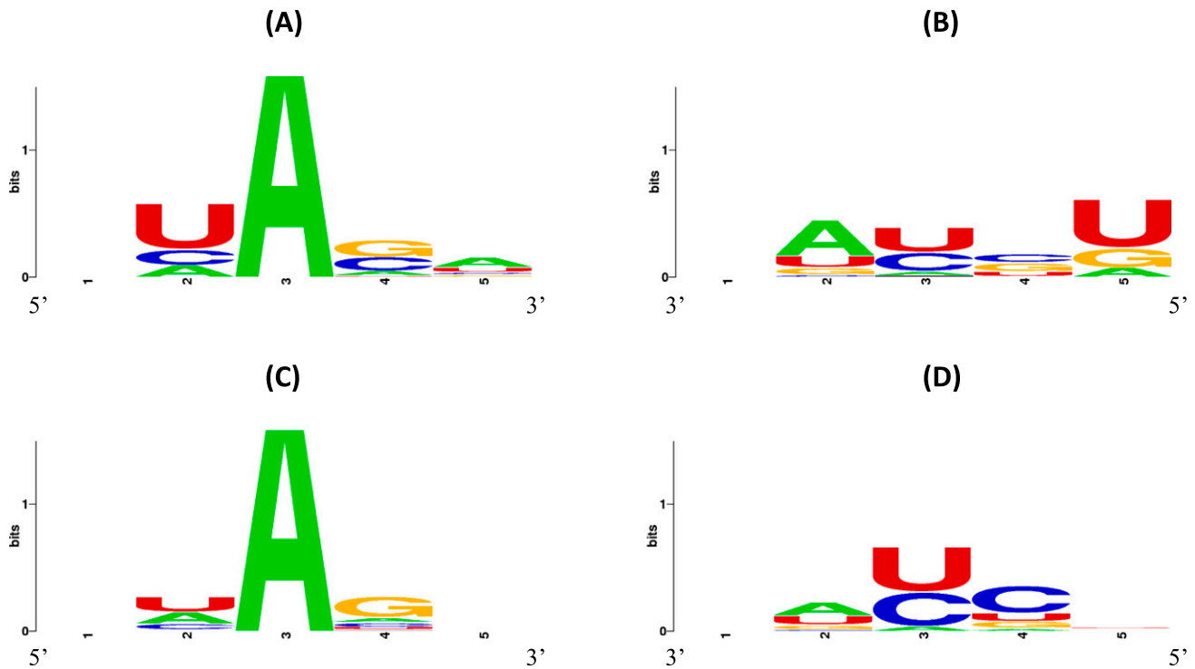
Figure 2. Sequence preference in the bases flanking the A-to-G editing sites detected in the human brain samples (A) and the mouse brain samples (C), in sequence Logo format (Crooks et al. 2004). (B,D) Sequence preference in the bases opposing the A-to-G editing sites for the human brain samples and the mouse brain samples, respectively.
