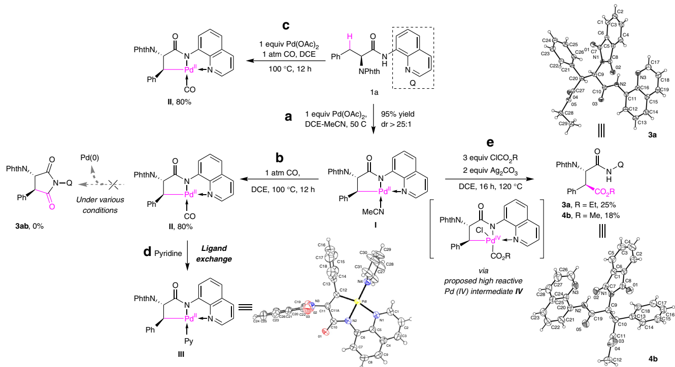
Figure 2 | Proof of concept on alkoxy-carbonylation of methylene C(sp 3 )-H bonds via Pd(II)/Pd(IV) catalysis. (a) Synthesis of palladacycle I . (b) Stoichiometric reaction of palladacycle I with carbon monoxide. (c) Synthesis of CO-coordinated Pd(II) complex II . (d) Structure confirmation of complex II via the transformation to complex III . The structure of complex III was unambiguously confirmed by single-crystal X-ray diffraction. (e) Stoichiometric reaction of palladacycle I with ClCO 2 R. The structure of compounds 3a and 4b was confirmed by single-crystal X-ray diffraction.
