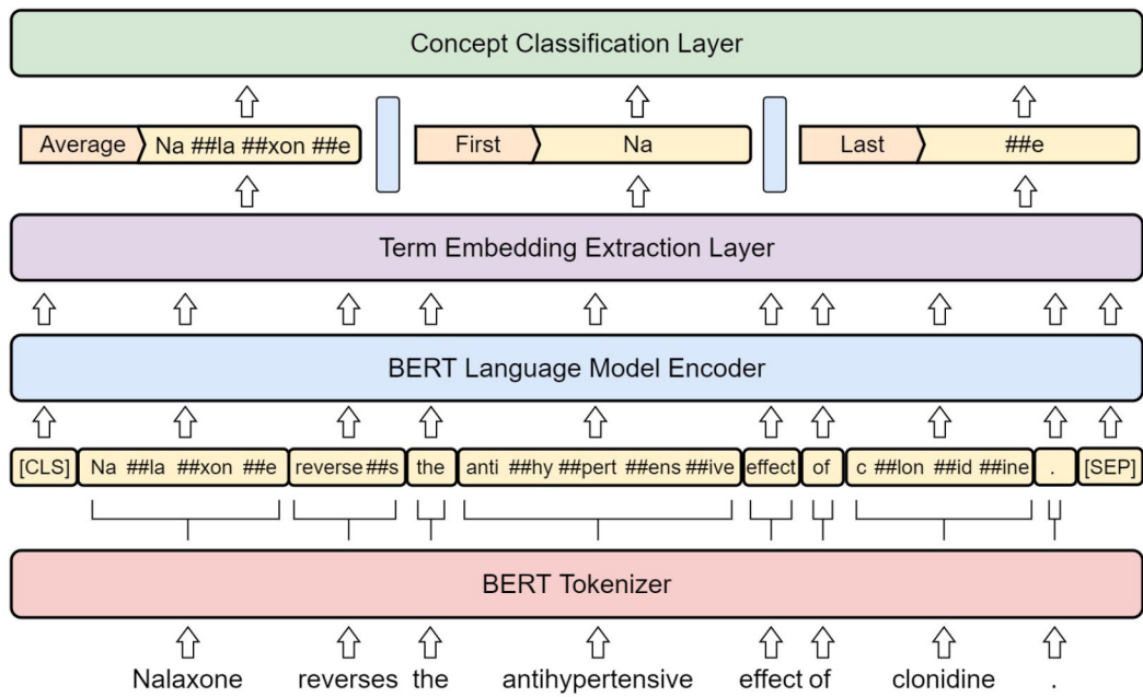
Figure 1: Named Entity Normalization (NEN) Model. This depiction demonstrates embedding context as the term’s sequence. We also explore two more context aggregation methods which are not shown.
