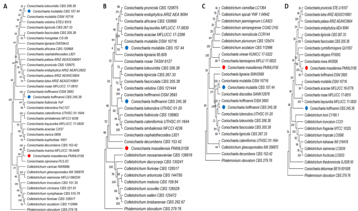
Figure 7. Four single-locus phylogenetic trees using the ITS (A), D1/D2 (B), B-tub2 (C), and TEF-1 \alpha (D) genomic regions. The species included in each tree differ because the sequences for each locus were not available for all strains. The red dots indicate the new species Coniochaeta massiliensis PMML0158 and blue dots indicate type strains. Phialemonium obovatum CBS 279.76 was used as the outgroup. The maximum-parsimony tree was generated using the MEGA 11 software, with 1000-replication bootstrap values.
