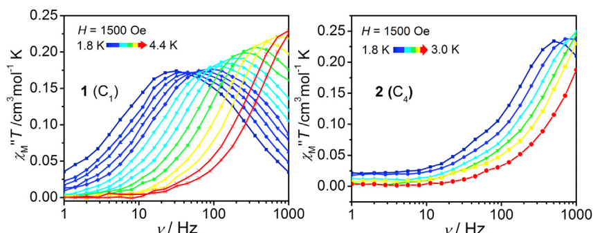
Figure 2. The Magnetic Relaxation of 1 and 2
