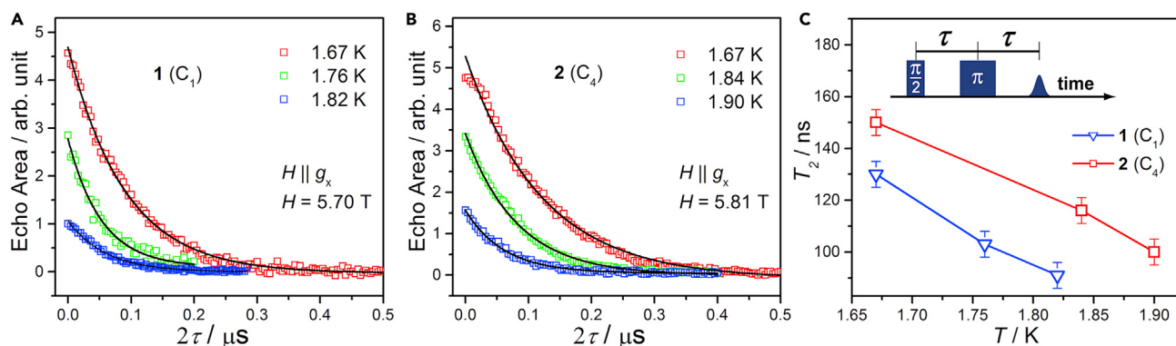
Figure 4. The Quantum Coherence of 1 and 2
