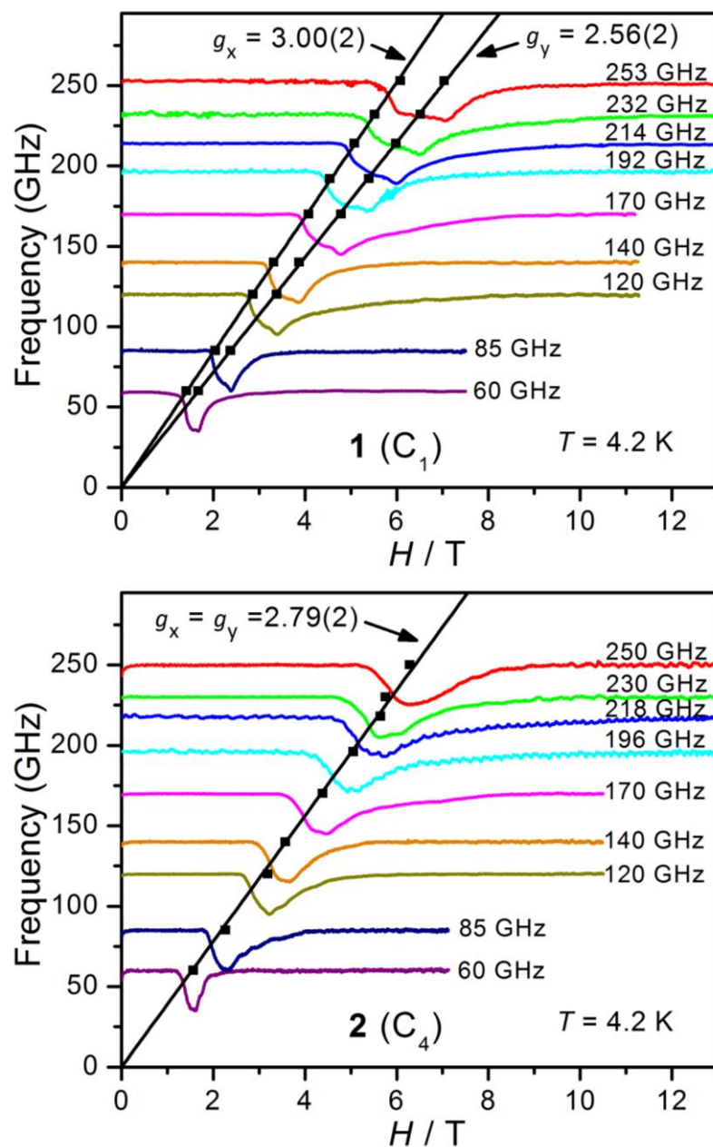
Figure S5. Variable-frequency EPR spectra collected on powder samples of 1 (top) and 2 (bottom) under 4.2 K. Solid lines are simulations of the frequency dependence of the peak positions employing the parameters given in the text. Related to Figure 2.
