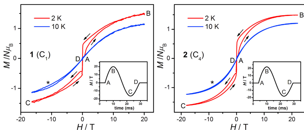
Figure 3. The Magnetic Hysteresis Loop of 1 and 2
