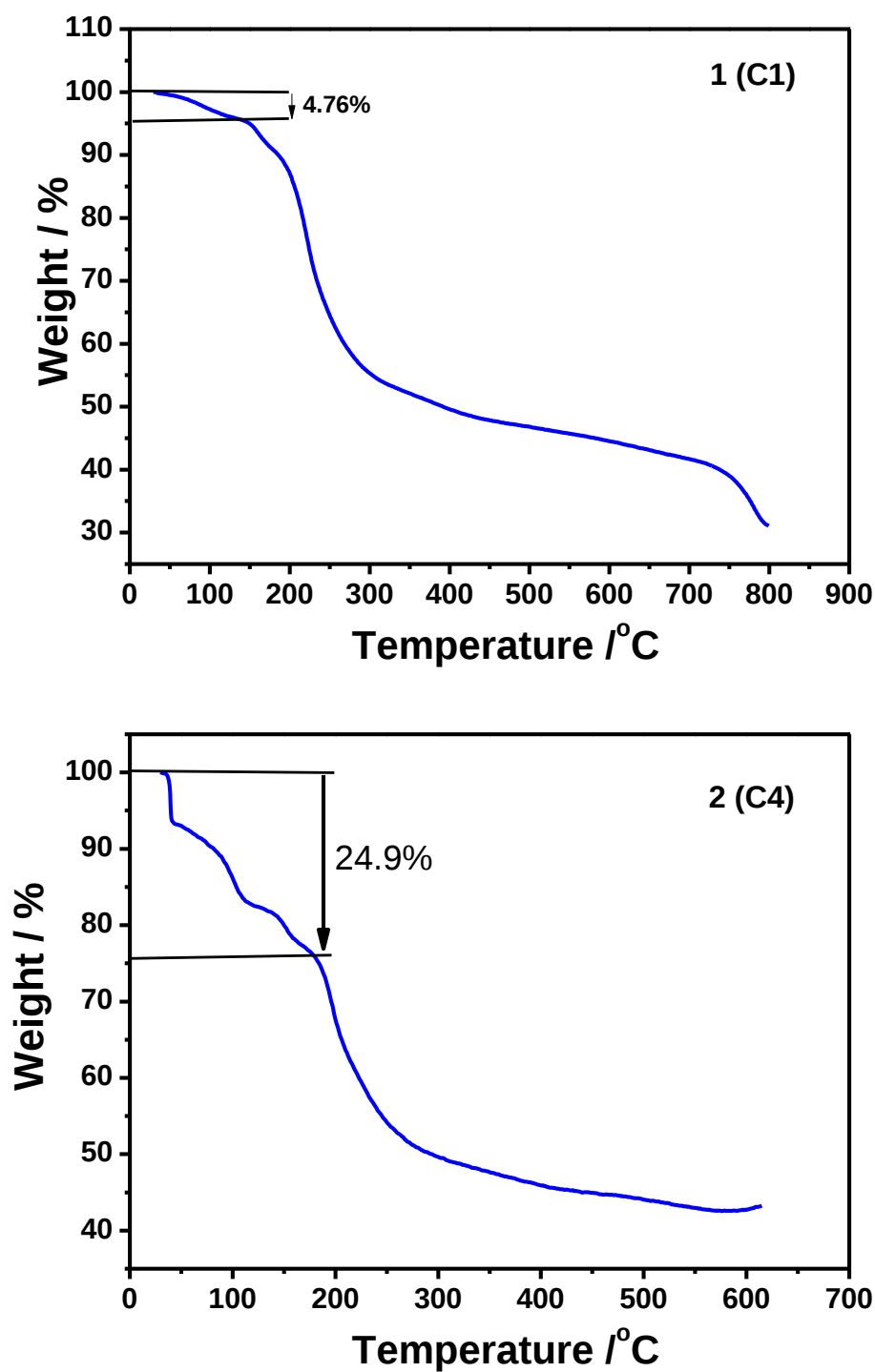
Figure S2. Thermogravimetric analysis of 1 (top) and 2 (bottom) in N 2 . The ramp rates were 10 °C min -1 for 1 from 25 to 800 °C and 5 °C min -1 for 2 from 25 to 615 °C. Related to Figure 1.
