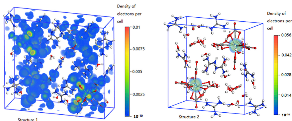
Figure 5. The Spatial Distributions of the Spin States of 1 and 2
