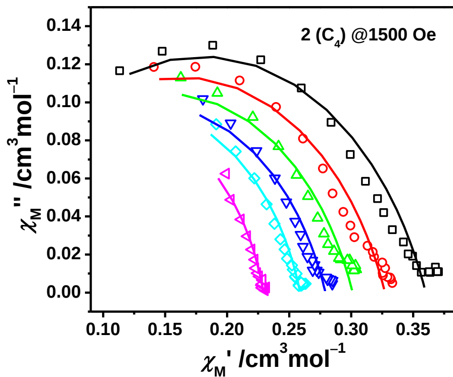
Figure S12. Variable temperature Cole-Cole plots under 1500 Oe dc field at indicated temperatures for complex 2 . Related to Figure 2.
