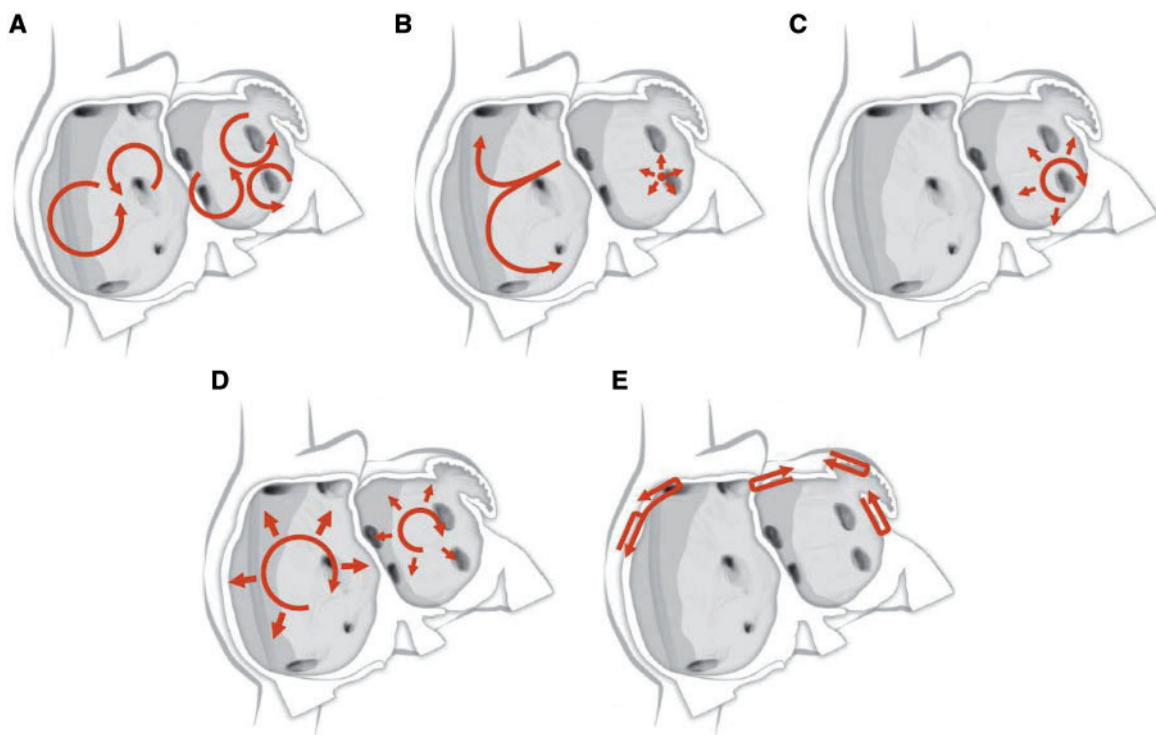
Figure 3 Schematic drawing showing various hypotheses and proposals concerning the mechanisms of atrial fibrillation. (A) Multiple wavelets hypothesis. (B) Rapidly discharging automatic foci. (C) Single reentrant circuit with fibrillatory conduction. (D) Functional reentry resulting from rotors or spiral waves. (E) AF maintenance resulting from dissociation between epicardial and endocardial layers, with mutual interaction producing multiplying activity that maintains the arrhythmia.
