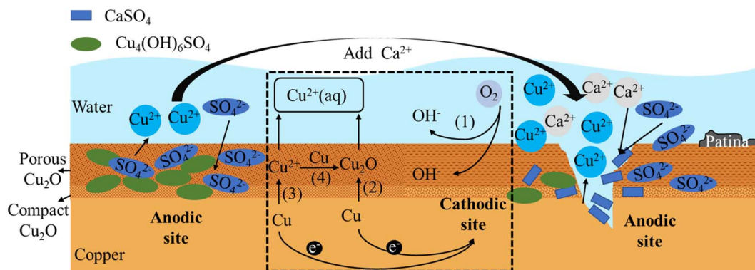
Fig. 9 Schematic diagram of copper corrosion and by-product release under \text{SO}_4^{2-} condition.
