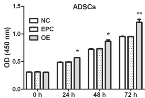
Figure 3. Klotho OE promotes the proliferation of ADSCs. NC, ADSCs group; EPC, ADSCs + empty plasmid control group; OE, ADSCs + klotho OE group. * P < 0.05 , ** P < 0.01 compared with EPC ( n = 3 ). OE, overexpression; ADSCs, adipose-derived stem cells; EPC, empty plasmid control group.
