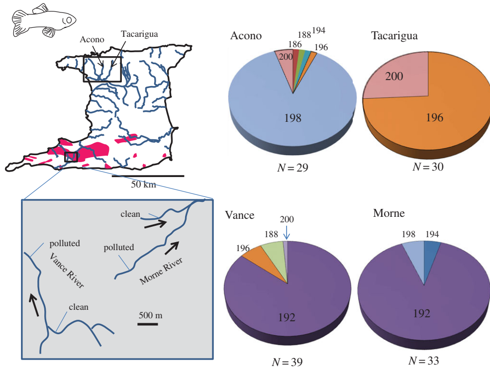
Figure 1. Distribution of alleles for a DNA microsatellite within the CYP1A gene for guppies living in four rivers in Trinidad. The Vance and Morne rivers are unconnected by freshwater and have stretches that are heavily contaminated with crude oil, described in [27]. Within each polluted river, data are pooled for populations from unpolluted and polluted stretches as no frequency differences were observed. Numbers within the pie charts are the sizes (bp) of each allele.
