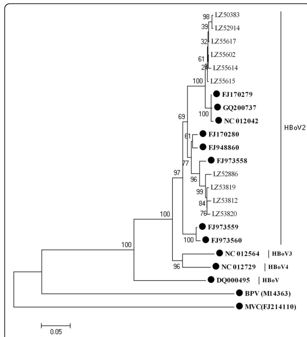
Figure 3 Phylogenetic analysis of the partial VP1 gene sequences of human bocavirus1-4 and other bocavirus members. Phylogenetic tree was constructed by the neighbor-joining method, Kimura 2-parameter model with 1,000 bootstrap replicates, by using MEGA 4.1 package. Black dots designate reference strains, the others were sequences generated from the present study. MVC: Minute virus of canines; BPV: Bovine parvovirus.
