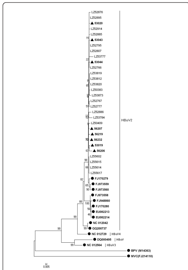
Figure 1 Phylogenetic analysis of human bocavirus1-4 and other bocavirus members partial NS1 gene sequences. Phylogenetic tree was constructed by the neighbor-joining method, Kimura 2-parameter model with 1,000 bootstrap replicates, by using MEGA 4.1 package. Black dots designate reference strains, black triangles designate sequences from control group and the others were sequences generated from the gastroenteritis children in the present study. MVC: Minute virus of canines; BPV: Bovine parvovirus.
