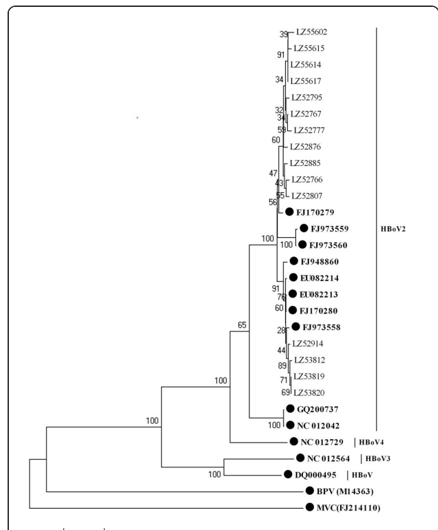
Figure 2 Phylogenetic analysis of the partial NP1 gene sequences of human bocavirus1-4 and other bocavirus members. Phylogenetic tree was constructed by the neighbor-joining method, Kimura 2-parameter model with 1,000 bootstrap replicates, by using MEGA 4.1 package. Black dots designate reference strains, the others were sequences generated from the present study. MVC: Minute virus of canines; BPV: Bovine parvovirus.
