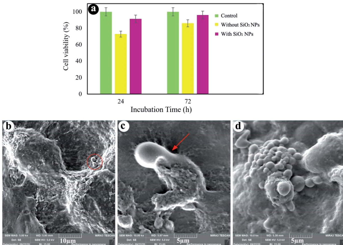
Fig. 6 Cell viability (a), FE-SEM images of cell-cultured hydrogels with 3.0% SiO 2 (b and c) and without SiO 2 (d).
