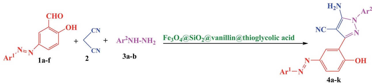
Scheme 2 Synthesis of novel azo-linked 5-amino-pyrazole-4-carbonitrile 4a-k using of \text{Fe}_3\text{O}_4@SiO_2@vanillin@thioglycolic\ acid .
