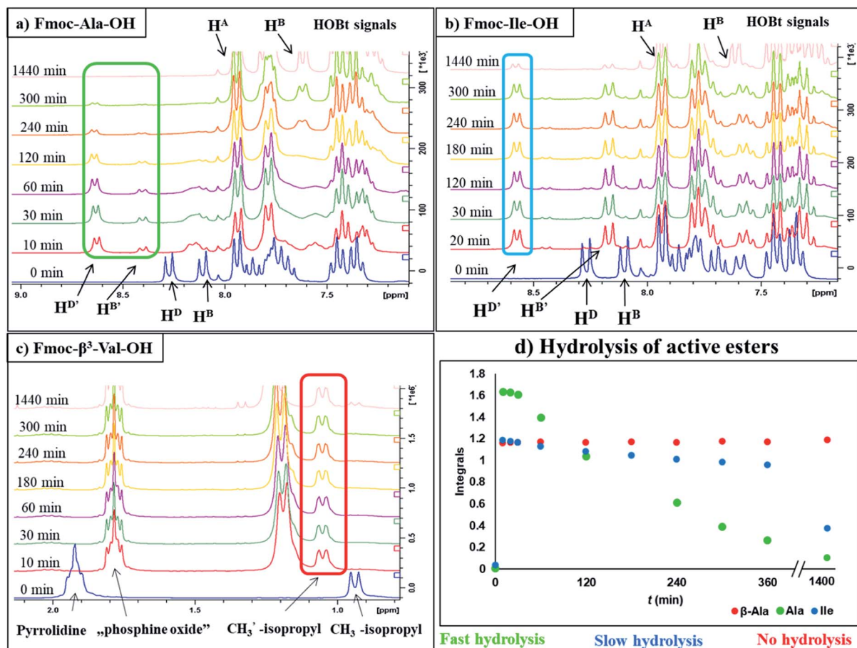
Fig. 1 ^1\text{H} NMR resonance frequency and intensity changes as a function of the time ( T = 25^\circ\text{C} ) during the active ester formation and hydrolysis of the three different groups of amino acids. Selected ^1\text{H} -resonances (e.g. \text{H}^{\text{D}'} , \text{H}^{\text{B}'} as the aromatic ring protons of active ester or \text{H}^{\text{D}} as the side chain protons of active ester) are used to monitor and analyze the kinetics of the reactions. (a) NMR spectra of the quickly hydrolyzed active ester from Fmoc-Ala-OH with PyBOP, (b) NMR spectra of the slowly hydrolyzed active ester from Fmoc-Ile-OH with PyBOP, (c) NMR spectra of the stable active ester from Fmoc- \beta^3 -Val-OH with PyBOP, (d) the integral–time diagram of three different group of amino acids referenced to the signal of DMF- d_7 : residue of fast hydrolyzing property is reported in green, while slow hydrolysis is depicted with blue and non-hydrolyzing residue with red.
