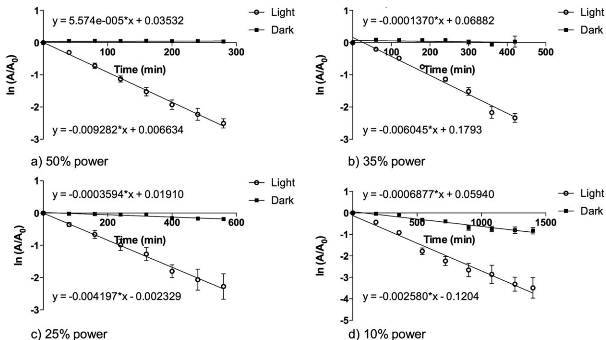
FIGURE 5. First order plots for reduction in ADPA absorbance by ^1O_2 produced from TMPyP-incorporated HEMA:MMA:MAA polymer at 378 nm following either irradiance using the white halogen source or dark conditions with varying power and total times. The power outputs and time points used in the experiment were as follows: (a) 50% power ( 3.02 \text{ mW/cm}^2 ) - 40, 80, 120, 160, 200, 240, 280 min; (b) 35% power ( 2.114 \text{ mW/cm}^2 ) - 0, 60, 120, 180, 240, 300, 360, 400 min; (c) 25% power ( 1.51 \text{ mW/cm}^2 ) - 80, 160, 240, 320, 400, 480, 560 min; (d) 10% power ( 0.604 \text{ mW/cm}^2 ) - 0, 180, 360, 540, 720, 900, 1080, 1260, 1400 min, where A is the absorbance at time t and A_0 is the absorbance at time 0.
