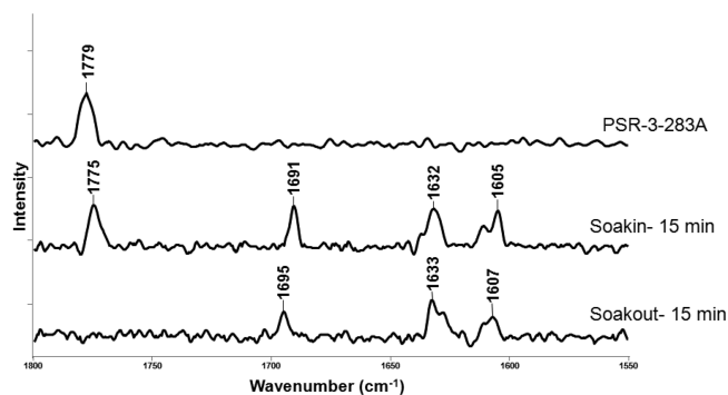
Figure 5. Soak-in and soak-out reactions of PSR-3-283A in crystals of SHV-1. One microliter of 20 mM PSR-3-283A was added to 4\ \mu\text{L} of holding solutions containing a SHV-1 crystal. Raman spectra were recorded at different time points. After 15 min, the crystal was transferred to a fresh drop that did not contain the PSR-3-283A inhibitor. Raman spectra were taken at different time points. The spectra shown in the figure are 15 min after PSR-3-283A was soaked in (middle) and 15 min after the SHV-1 crystal was transferred out to the holding solution (bottom).
