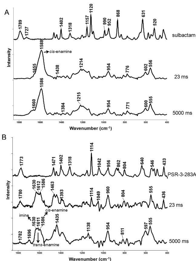
Figure 3. Raman studies of reactions with SHV-1 in solution. The SHV-1 (2 mg/mL) was mixed with sulbactam (A) or PSR-3-283A (B) at the molar ration of 1:10 (E/I). Using the KinTek device, the reaction was quenched at different time points from 23 ms to 1 min. The quenched samples were then freeze-dried, and their Raman spectra were recorded.
