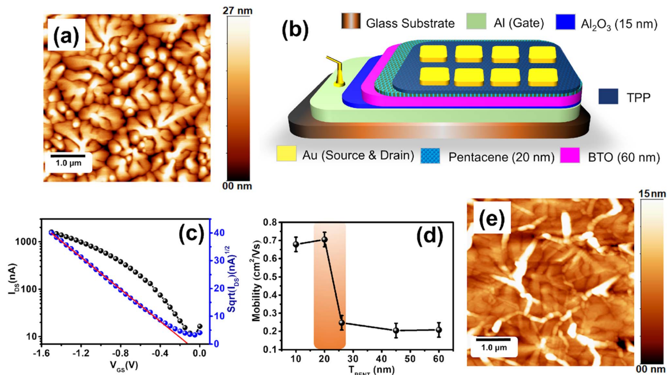
Fig. 1 (a) Surface morphology of the pentacene film showing the grain boundaries of the dendrite structures. (b) Schematic diagram of the OFET. (c) Transfer characteristic of the 20 nm pentacene film-based OFET. (d) Variation of mobility of the pentacene film grown on BaTiO 3 /Al 2 O 3 /Al/Glass. A 20 nm pentacene film was selected for the sensing experiment due to higher field-effect mobility. (e) Surface morphology of the peptide film (5000 rpm coated) on a pentacene film.
