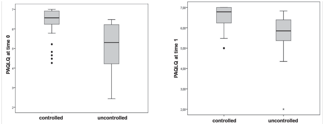
Figure 1 Differences in HRQL between controlled and uncontrolled patients at the first visit ( p < 0.01 ) and at the second visit ( p < 0.001 ).
