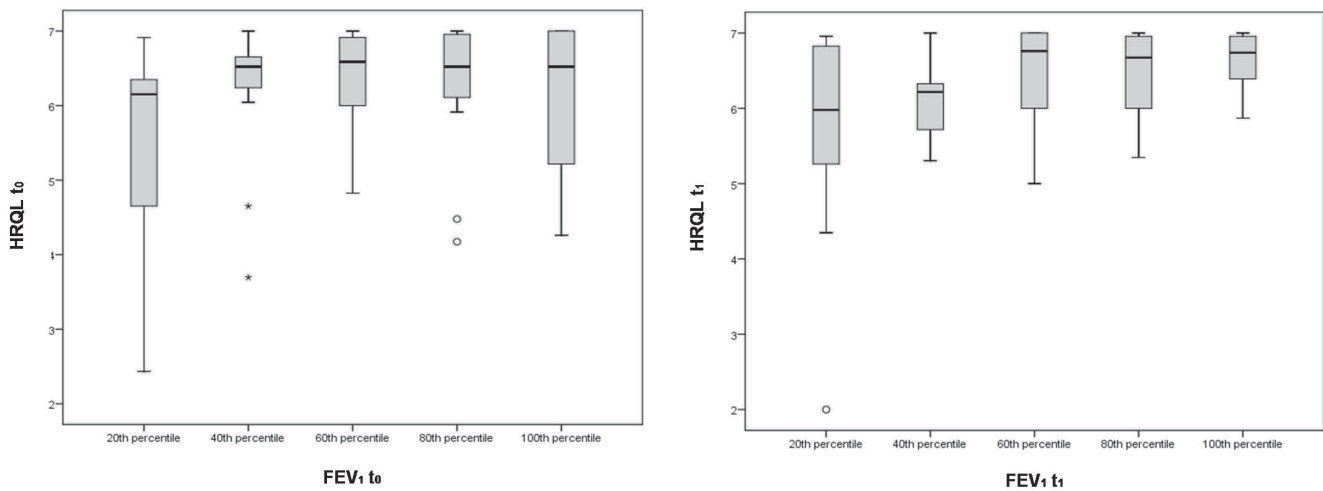
Figure 3 Median HRQL score trend in function of FEV 1 values at t 0 (on the left) and at t 1 (on the right). Boxes are delimited by the 25 th percentile (at the bottom) and 75 th percentile (top) of HRQL.
