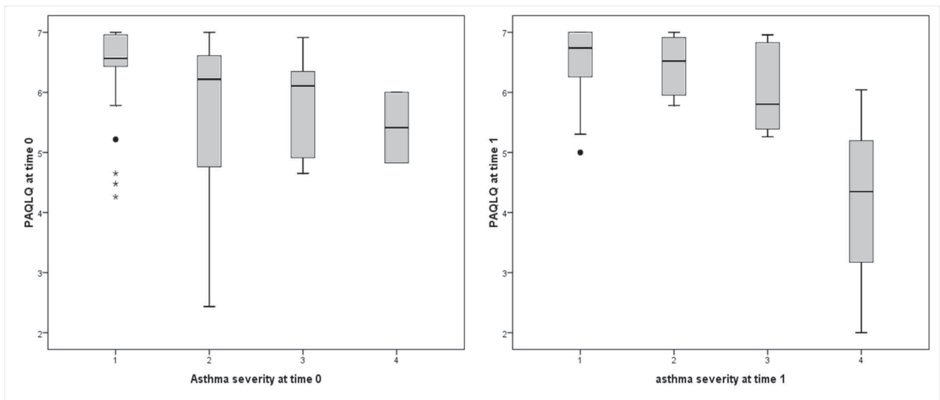
Figure 2 Decrease in the PAQLQ score in patients with increasing asthma severity at time 0 and at time 1 ( p < 0,04 at time 0 and p < 0,03 at time 1).
