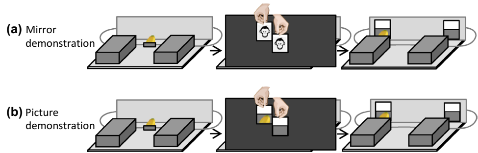
Fig. 7 Experiment 5: illustration of the setup from the subjects' perspective. Subjects were presented either with mirrors (a) or pictures of the final mirror images (b) while the platform was occluded. In the final stage of the procedure, subjects saw either two mirrors or pictures of the mirror images (independent of the cue type shown before)
