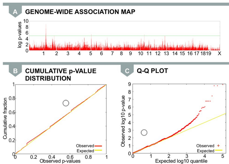
Fig 4. Expected distribution of p -values in a typical (A) Manhattan plot, (B) cumulative p -value distribution, and (C) Q-Q plot. Circles in (B) and (C) denote where the median p -value (red line) falls on the graph in comparison to the expected median p -value (yellow line). Here, the median falls close to 0.5, suggesting that population structure is not affecting association results or has been corrected for in the model. Q-Q, quantile-quantile.
