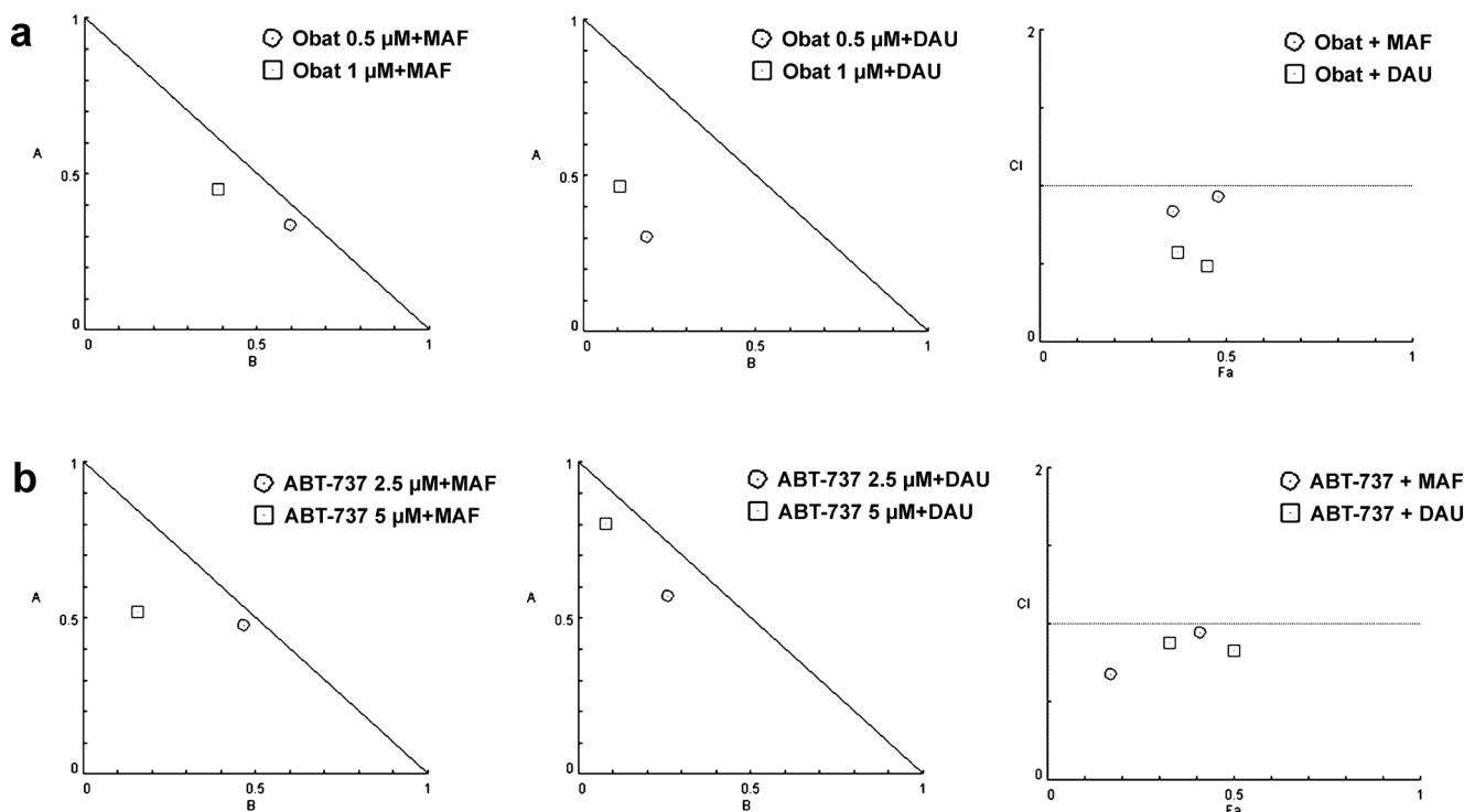
Fig. 3 The CI values corresponding to the obatoclox or ABT-737 combinations with mafosfamide or daunorubicin were determined by isobologram analysis. A representative normalized isobolograms and fraction affected (Fa)-CI plots generated for HL-60 cells exposed to the
