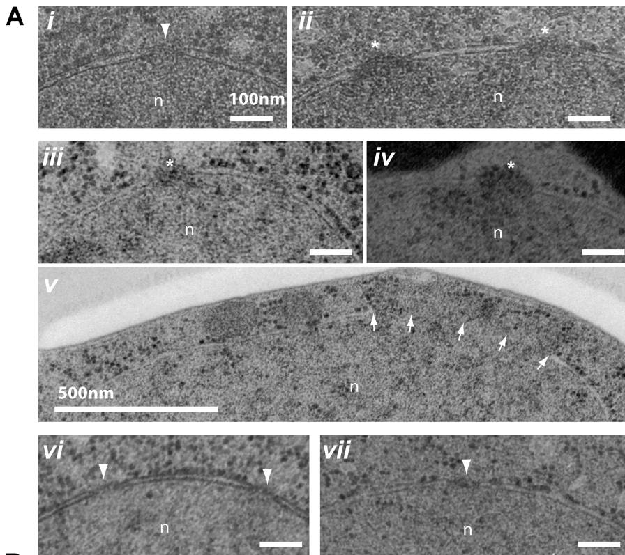
Figure 7. Transmission EM analysis of NPC morphology in conditional mutants affecting Ndc1-interacting nucleoporins. (A) NPCs (arrowheads) in pom152Δ pom34Δ GAL-3×HA-NUP59 cells in permissive conditions (i) did not display morphological abnormalities. (ii) After incubation in nonpermissive conditions, a large fraction of dilated pores often displaying fuzzy electron-dense material could be detected (asterisks). (iii) A similar phenotype was observed in pom152Δ pom34Δ nup53Δ MET3-3×HA-NUP59 cells in permissive conditions. After incubation in nonpermissive conditions, these cells displayed not only dilated pores (iv) but also large openings in NE (v, arrows). In nup53Δ nup59Δ GAL-3×HA-POM34 cells, no obvious NPC size abnormalities could be detected both in permissive (vi) and nonpermissive conditions (vii). n, nucleus. Bars: (i–iv, vi, and vii) 100 nm; (v) 500 nm. (B, i–iii) Comparison of pore size distributions in pom152Δ pom34Δ GAL-3×HA-NUP59 cells (i), pom152Δ pom34Δ nup53Δ MET3-3×HA-NUP59 cells (ii), and nup53Δ nup59Δ GAL-3×HA-POM34 cells (iii) incubated in permissive and nonpermissive conditions. (iv) Comparison of pore numbers per section in nup53Δ nup59Δ GAL-3×HA-POM34 in either permissive or nonpermissive conditions. Gal, galactose medium; dex, dextrose-containing medium; –met, medium lacking methionine; 10× met, medium containing 10× methionine. Error bars indicate SEM.
