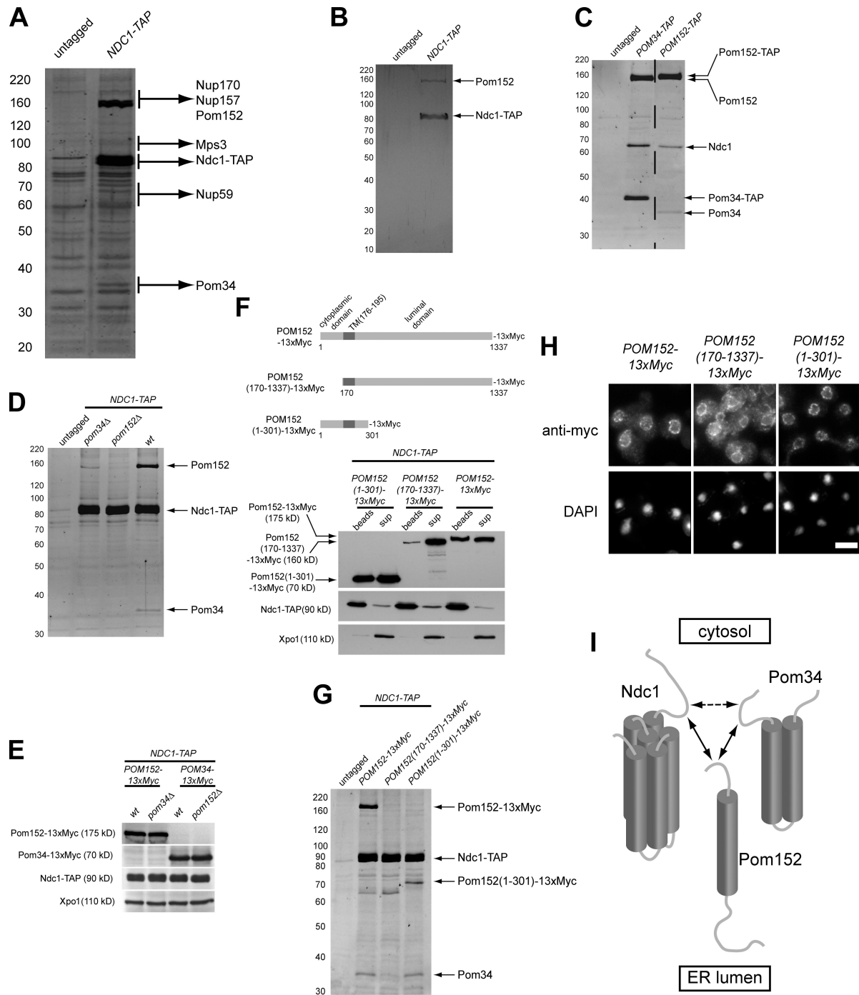
Figure 1. Identification of Ndc1-interacting proteins and characterization of the Ndc1 subcomplex. (A) Affinity purification from yeast expressing TAP-tagged Ndc1 ( NDC1-TAP ) or untagged controls. Gel areas were excised and subjected to LC-MS/MS. Lines mark borders of areas subjected to MS analysis. (B) Profile of an Ndc1 affinity purification performed in low ionic strength conditions. (C) Comparison of purifications performed from cells expressing TAP-tagged versions of Pom34 ( POM34-TAP ), Pom152 ( POM152-TAP ), or untagged controls. (D) Comparison of Ndc1-TAP affinity purifications from wild-type (wt), pom34Δ , pom152Δ , or untagged control cells. For A–D, purified proteins were eluted, separated by SDS-PAGE, and visualized by SYPRO-Ruby. (E) Western blot analysis of the levels of myc-tagged Pom152 or myc-tagged Pom34 in wild-type, pom34Δ , or pom152Δ cells expressing Ndc1-TAP. Ndc1-TAP and Xpo1/Crm1 levels are used as loading controls. (F) Western blot analysis of Ndc1 purifications from cells expressing Ndc1-TAP together with either 13xmyc-tagged Pom152 full-length , Pom152 170-1337 , or Pom152 1-301 . The scheme depicts the membrane topology of Pom152. Xpo1 was included as a control. sup, supernatant. (G) Comparison of Ndc1 purifications from cells expressing full-length Pom152-13xmyc or its truncations. Proteins were visualized with SYPRO-Ruby. (H) Distribution of full-length Pom152 and its truncations tagged with 13xmyc analyzed by immunofluorescence. Nuclei were stained with DAPI. (I) Model summarizing the interactions between Ndc1, Pom152, and Pom34. Solid arrows indicate direct protein interactions. The dashed arrow displays the functional requirement of Pom34 for the Ndc1 subcomplex integrity. Migration rate references for all gel image panels are shown in kilodaltons. Bar, 5 μm.
