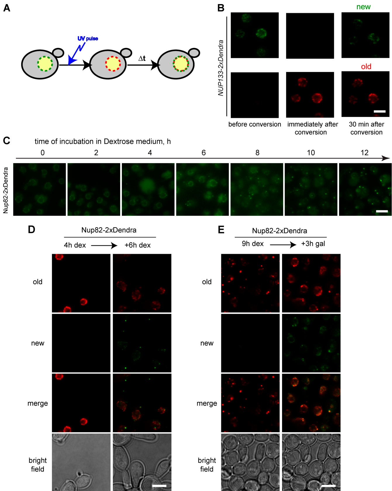
Figure 8. Dendra assay to analyze distribution of nucleoporins in nup53Δ nup59Δ GAL-3xHA-POM34 cells. (A) Representation of the use of Nup-Dendra fusions to track the localization of newly synthesized and preexisting nucleoporins. Initially, Dendra displays green fluorescence but can be irreversibly photoconverted into a red fluorophore by a short pulse of UV light. After conversion, newly made nucleoporins are detected in the green channel, whereas red fluorescence can be used to localize Nups that were synthesized before the photoconversion. (B) Distribution of red and green Nup133-2xDendra variants before (left), immediately after (middle), and 30 min after photoconversion (right). (C) Time course to visualize the Nup82-Dendra distribution in
