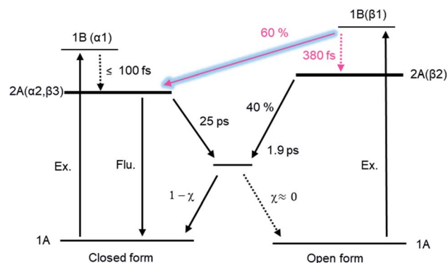
Fig. 9 Electrocytic reaction mechanism of DTA.
