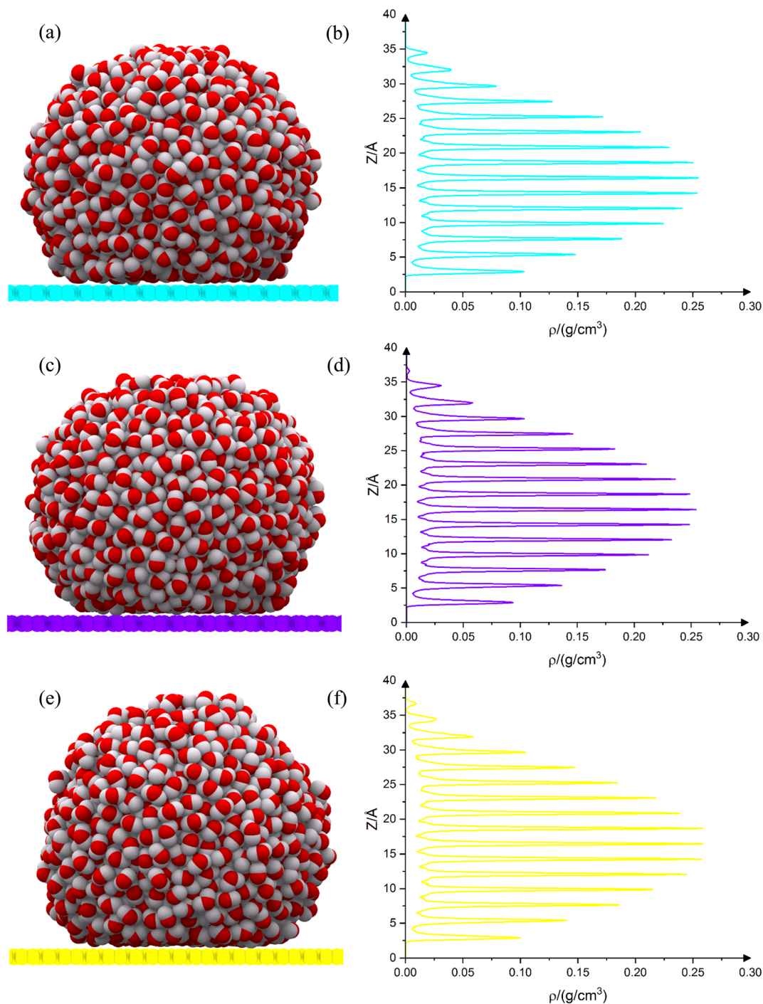
Fig. 4 Droplet equilibrium shape on net C (a), net W (c) and net Y (e). The carbon atoms in net C, net W and net Y are shown in cyan, violet and yellow colors, respectively. Droplet density diagram is along the Z axis for net C (b), net W (d) and net Y (f). The droplets on all three substrates are completely layered. The density diagram confirms this fact. Layer thickness on all three substrates is almost the same and is equal to 2.24 Å. The number of peaks in net C is equal to 15, but on net W and net Y is equal to 16, which is to the result of carbon atoms' surface density.
