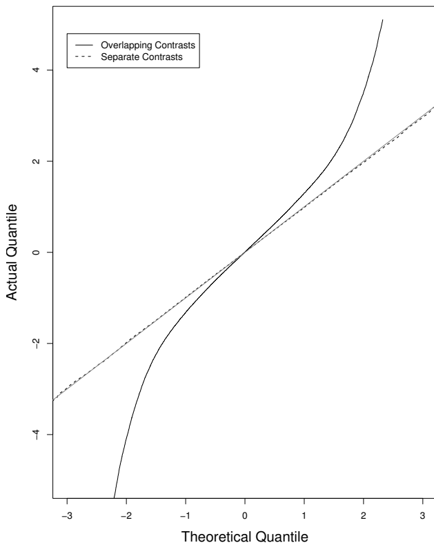
Figure 3 (Dependency of Calls) The density of \sqrt{n}(p_{AB} - E[p_{AB}])/(E p_{AB} - E[p_{AB}^2]) is compared to a N(0,1) density for 500 subject samples in a quantile-quantile plot. The deviation from the Y = X line indicates that n\hat{p}_{AB} is not distributed as a binomial( n, p_{AB} ) variable.
