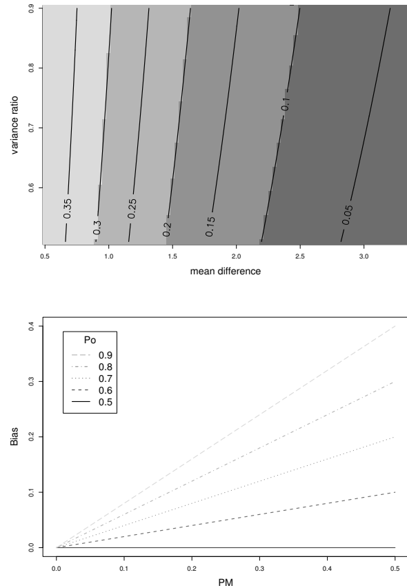
Figure 1 ( P_M and Bias) a) P_M depends on the ratio, \sigma_1^2 : \sigma_0^2 (y-axis) and on the difference, \mu_1 - \mu_0 (x-axis) b) The bias, p_0^* - p_0 (y-axis) depends on P_M (x-axis), and is shown for different values of p_0 .
