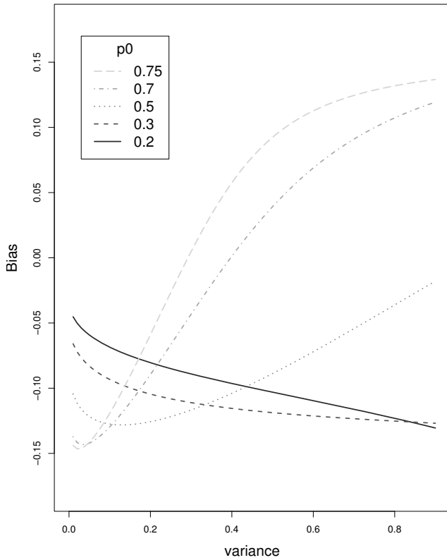
Figure 2 ( P_0 and Bias) The bias of the estimate, p_0^* = \lim_{n \rightarrow \infty} \sum_{i=1}^n 1(G^i = 0) / n , depends on p_0, \mu_1, \mu_2, \sigma_0^2 and \sigma_1^2 . After fixing, \mu_0 = 0, \sigma_0^2 = 1 , and \mu_1 = 1 , we plot the bias, p_0^* - p_0 (y-axis), against \sigma_1^2 (x-axis), for different values of p_0 .
