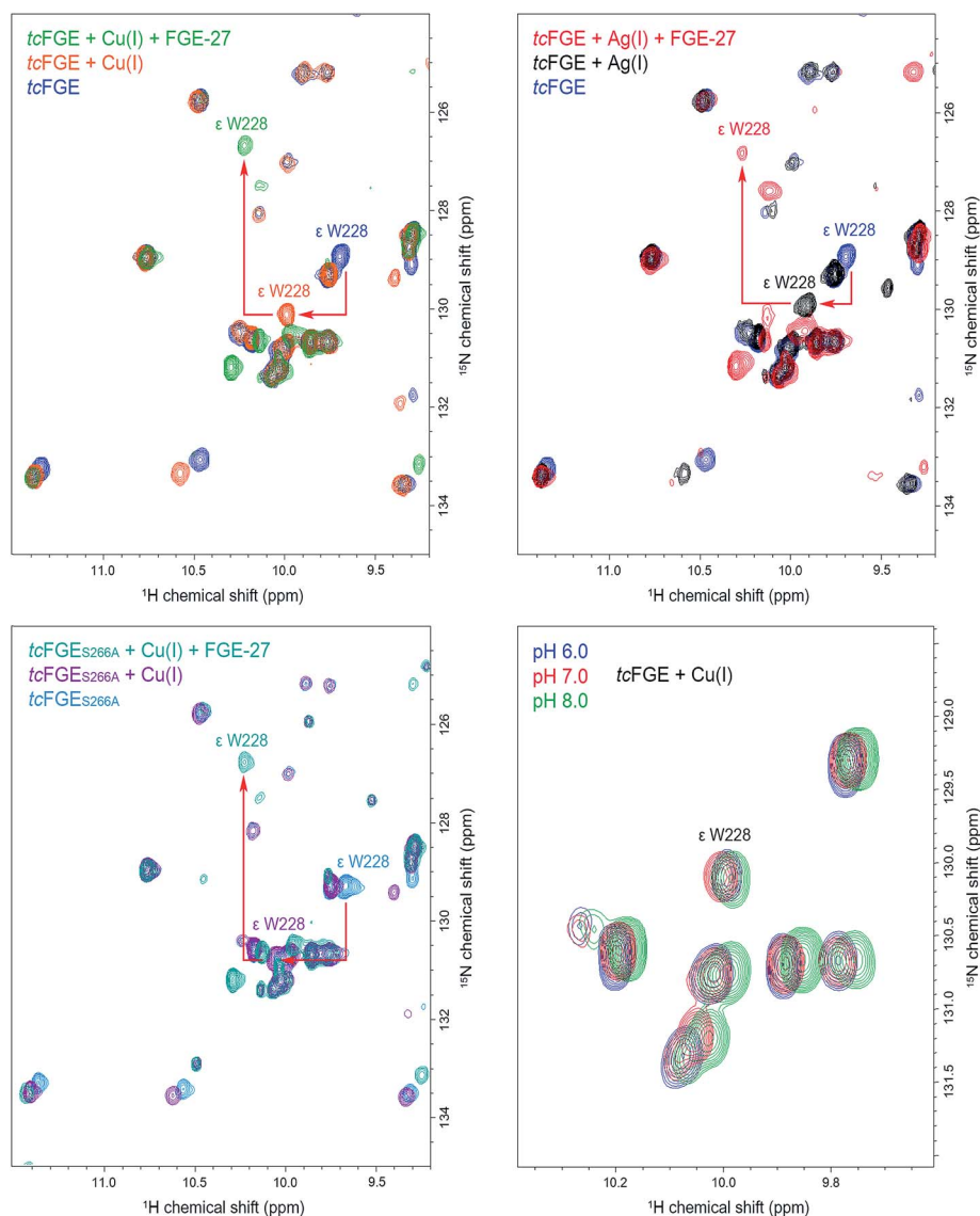
Fig. 4 ^1H - ^{15}N TROSY HSQC spectra of uniformly ^{15}N -labelled 300 \mu M tc FGE in 20 mM phosphate buffer, 50 mM NaCl, 2 mM DTT, 25 C. The downfield area of the amide region is presented. Top left: The overlay of the spectra of apo-form tc FGE, pH 8.0 (dark blue), tc FGE in the presence of 450 \mu M CuSO_4 , pH 8.0 (orange), tc FGE in the presence of 450 \mu M CuSO_4 and 1 mM FGE-27, 2 mM glucose, 2 units (U) glucose oxidase (GO), 200 U catalase (CAT), pH 8.1 (green). Top right: The overlay of the spectra of apo-form tc FGE, pH 8.0 (dark blue), tc FGE in the presence of 450 \mu M AgNO_3 , pH 8.0 (black), tc FGE in the presence of 450 \mu M AgNO_3 and 1 mM FGE-27, 2 mM glucose, 2 U GO, 200 U CAT, pH 8.1 (red). Bottom left: The overlay of the spectra of apo-form tc FGE S266A , pH 8.0 (blue), tc FGE S266A in the presence of 450 \mu M CuSO_4 , pH 8.0 (magenta), tc FGE S266A in the presence of 450 \mu M CuSO_4 and 1 mM FGE-27, 2 mM glucose, 2 U GO, 200 U CAT, pH 8.1 (dark cyan). Bottom right: The overlay of the spectra of tc FGE in the presence of 450 \mu M CuSO_4 measured at different pH.
