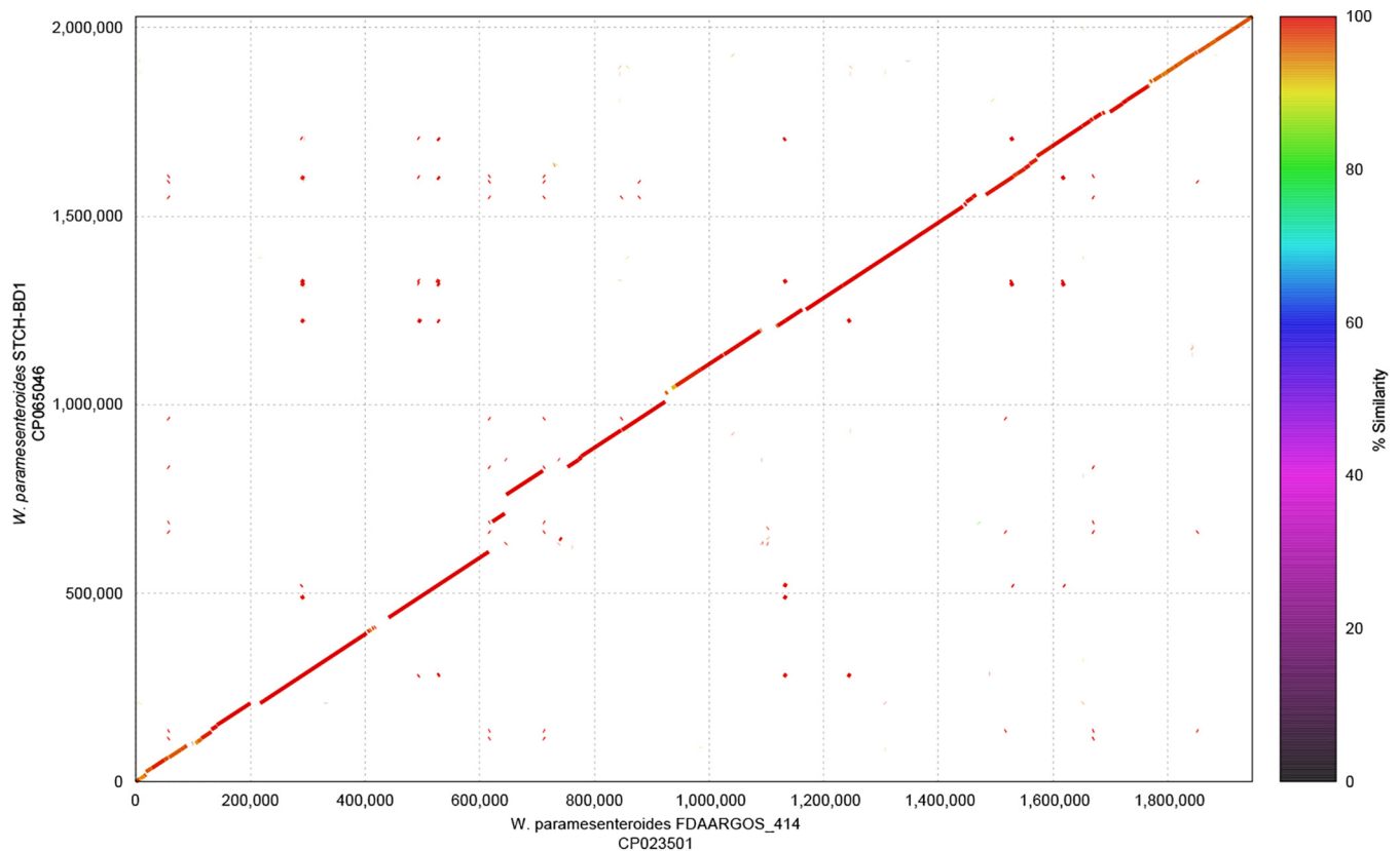
FIG 1 Genome alignment between Weissella paramesenteroides STCH-BD1 (GenBank accession number CP065046 ) and Weissella paramesenteroides FDAARGOS_414 ( CP023501 ) chromosomes. Percentage similarities are displayed using a rainbow color scale.
