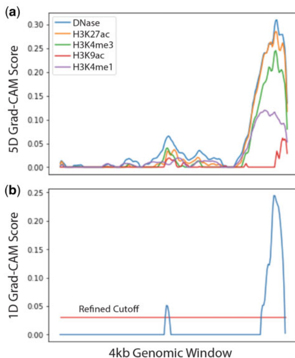
Fig. 6. Feature-wise and Position-wise Grad-CAM Values: (a) 5-D and (b) 1-D Grad-CAM justification of a positive prediction
