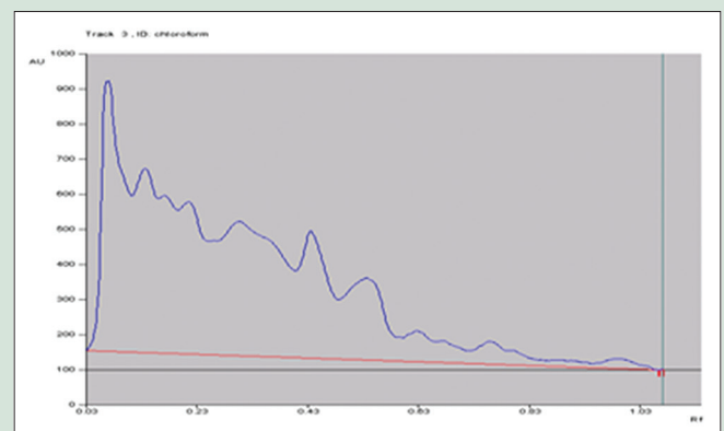
Figure 5: High-performance thin layer chromatography densitogram of Qurse Tabasheer at 366 nm chloroform extract
