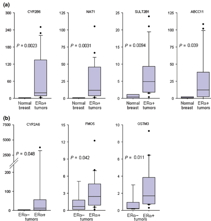
mRNA expression levels of the seven selected genes. (a) Comparison between normal breast versus estrogen receptor alpha (ER \alpha )-positive breast tumors. (b) Comparison between ER \alpha -negative versus ER \alpha -positive breast tumors. P value, Mann-Whitney test. Box central bar, median mRNA level.
