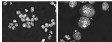
The nuclei of ES cells lacking Smc2 (right) are large and misshapen.
