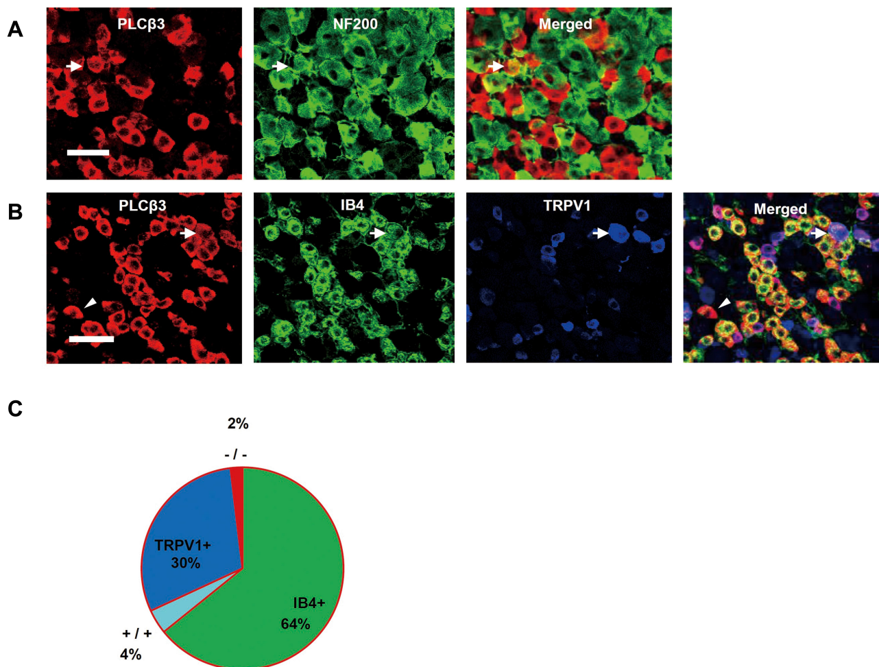
Figure 1 Expression of PLC \beta 3 in DRG neurons of naïve mice. (A) Co-localization of PLC \beta 3 (red) with NF200 (green). PLC \beta 3 immunoreactivity was found in small- to medium-sized DRG neurons. Most of the PLC \beta 3-positive profiles were NF200-negative. An arrow indicates both a PLC \beta 3-positive and an NF200-positive neuron. Scale bar = 50 \mu m. (B) Co-localization of PLC \beta 3 (red) with IB4 (green) and TRPV1 (blue). Many of the PLC \beta 3 immunoreactivity profiles were IB4-positive and/or TRPV1-positive profiles. 52% of TRPV1-expressing DRG neurons were PLC \beta 3-positive. An arrow indicates PLC \beta 3 immunoreactivity found in an IB4-positive/TRPV1-positive profile. An arrowhead indicates PLC \beta 3 immunoreactivity found in an IB4-negative/TRPV1-negative profile. Scale bar = 50 \mu m. (C) A pie chart summarizing the co-localization of PLC \beta 3 with IB4 and TRPV1. The chart shows that 64%, 30% and 4% of the PLC \beta 3-expressing DRG neuron profiles were IB4-positive, TRPV1-positive, and both IB4- and TRPV1-positive, respectively. Data were calculated using combined data from 4 mice (1571 PLC \beta 3-positive profiles from 4 mice).
