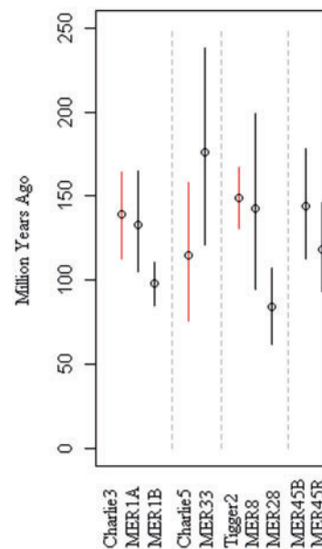
FIG. 5. Comparison of the time to element MRCA for related transposon families. Time to element MRCA, for each transposon family, predicted by BEAST using human–chimpanzee orthologs. Transposon families are grouped by likely homology and divided using a dashed line. Transposons marked in red contain a recognizable ORF.
