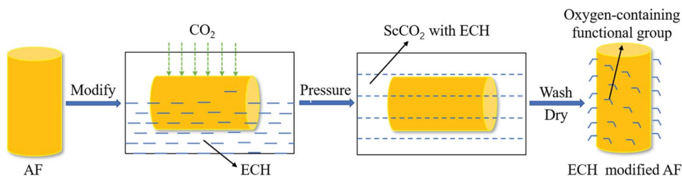
Fig. 2 Process diagram of the modification of the AF surface with ECH in \text{ScCO}_2 medium.
