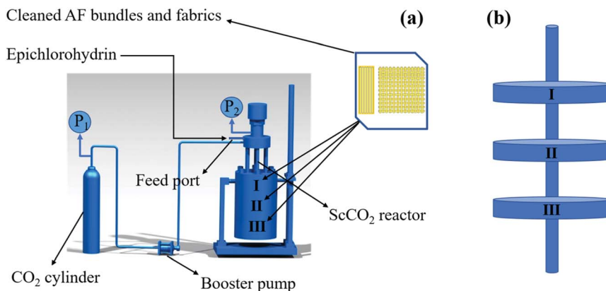
Fig. 1 Schematic diagram of the device containing AF surfaces treated with ECH in an \text{ScCO}_2 reactor (a) and the platform to fix the fiber (b).
