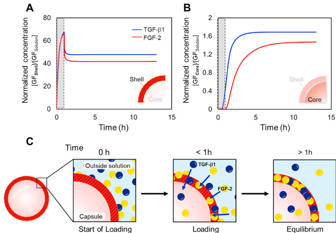
Fig. 6. Modeling GF concentration in the core and the shell of a microcapsule. Average concentration of GF (red: FGF-2, blue: TGF-β1) inside a microcapsule was normalized to solution concentrations used for GF loading (Table S2) and plotted as a function of time (h) for (A) hydrogel shell and (B) aqueous core. The gray box indicates loading time of 1 h. (C) Schematic illustration of GF incorporation and release mechanism.
