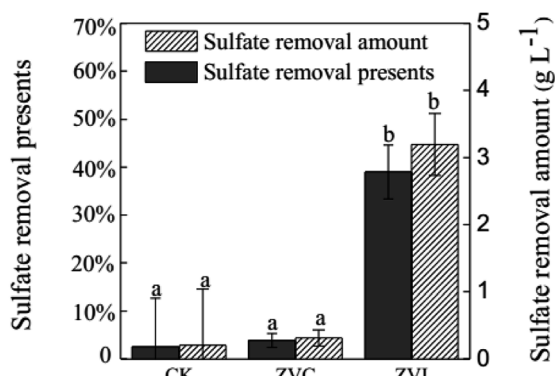
Fig. 5 Amount and percentage of sulfate removal in A. ferrooxidans system (ZVI) with or (CK) without zero-valent iron reduction, and (ZVC) with zero-valent copper reduction, respectively.
