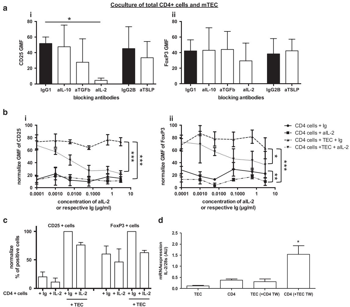
Figure 7 The protective effects of mTECs on Treg cell phenotype are mediated by IL-2. Purified CD4 + T cells were cultured alone or with mTECs for 3 days in the presence of different cytokines antagonists. (a) CD25 (i) and FoxP3 (ii) GMF expression in CD4 cells in different culture conditions were analyzed by flow cytometry (normalized data, n=3 ; mean \pm S.E.M.). The blocking antibodies against IL-10, TGF- \beta , and IL-2 were compared with their control isotype IgG1 and anti-TSLP was compared with its control isotype IgG2. (b) Purified CD4 + T cells were cultured alone or with mTECs for 3 days in the presence of increasing concentrations of IL-2 or its respective Ig. CD25 (bi) and FoxP3 (bii) GMF were assessed by flow cytometry ( n=3 , mean \pm S.E.M.). To avoid the inter-experiment variability, data from each experiment were analyzed thanks to Graphpad 'normalize' function, as described in Materials and methods. (c) The effects of IL-2 treatment (or its respective Ig) on the percentages of CD25 and FoxP3 + cells in the presence or absence of mTECs are reported in the graph. Statistical analyses were conducted using a two-way ANOVA test; * P < 0.05 , ** P < 0.005 , *** P < 0.001 . (d) mRNA expression of IL-2 in mTECs or CD4 + cells, alone or in coculture ( n=5 , mean \pm S.E.M.). Statistical analyses were conducted using a non-parametric t -test; * P < 0.05
