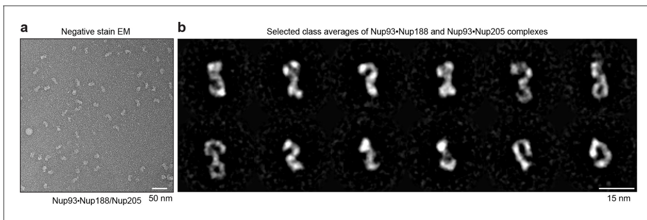
Figure 3. Structural analysis of natively purified Nup93 complexes. (a) Anti-Nup93 nanobody TP179-purified Nup93•Nup188 and Nup93•Nup205 complexes were subjected to the GraFix procedure (Kastner et al. , 2008) and negative staining for analysis by electron microscopy. (b) Gallery of 12 selected class averages of Nup93•Nup188 and Nup93•Nup205 particles.
