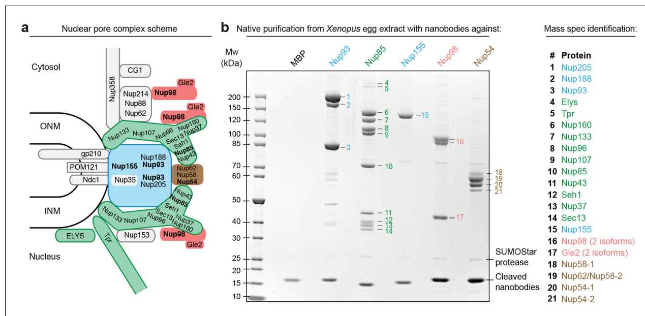
Figure 2. Purification and native elution of NPC subcomplexes with specific nanobodies. (a) Schematic representation of the subcomplex organization and relative localization of Nups within an asymmetric unit of the eightfold rotational symmetric vertebrate NPC (ONM/INM = outer and inner nuclear membrane). The nuclear and cytoplasmic rings of the structural NPC scaffold are mainly composed of the Nup107-Nup160 Y-shaped complex (green). The central inner ring of the scaffold is composed of the Nup93 subcomplex (blue). The scaffold is bound to the nuclear envelope via transmembrane Nups and further anchors FG-repeat nucleoporins (e.g. Nup98 [red] and the Nup62•Nup58•Nup54 complex [brown]) within the central channel, where they form the permeability barrier. Nups against which nanobodies were raised are highlighted in bold. (b) Native purification of major NPC scaffold subcomplexes and FG-repeat nucleoporins from Xenopus egg extract. Biotinylated His 14 -Avi-(GlySer) 9 -SUMOStar-(GlySer) 9 -tagged nanobodies were immobilized on magnetic Streptavidin beads and then incubated with Xenopus egg extract. After washing, nanobodies were gently eluted along with their bound target complexes by SUMOStar protease cleavage. One tenth of the eluates were analyzed by SDS-PAGE and Coomassie staining. All labeled bands were identified via mass spectrometry. The color code represents the subcomplex organization of the NPC as illustrated in (a). A nanobody raised against Escherichia coli Maltose-binding protein (MBP) served as a negative control. NPC, nuclear pore complex.
