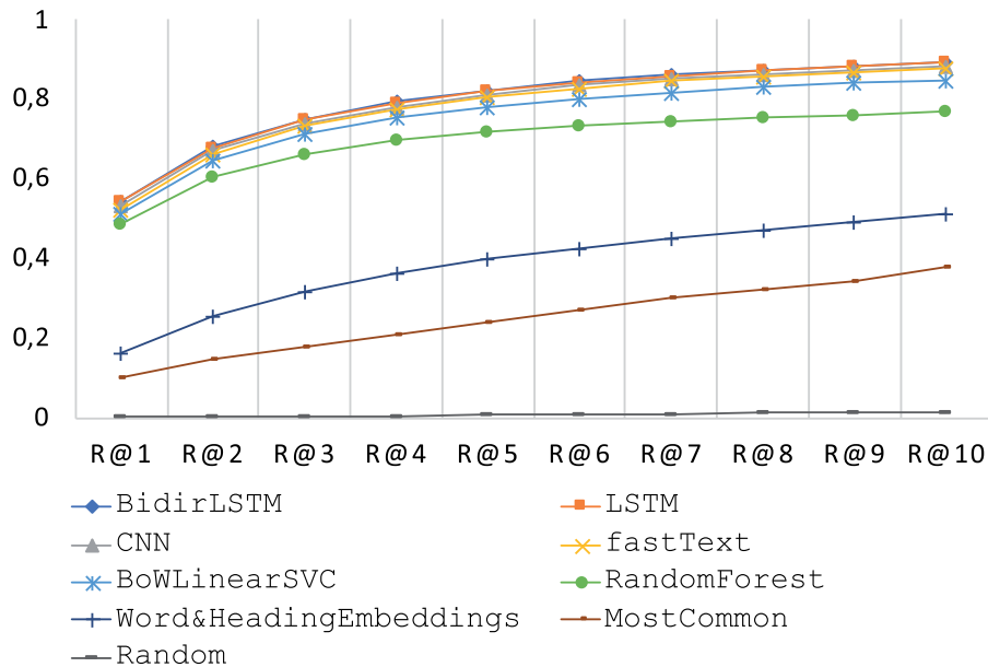
Figure 3. Recall at (R@) 1-10 plotted for each method. A high quality version of the plot for the top 6 performing methods is included in the Supplementary Appendix .
