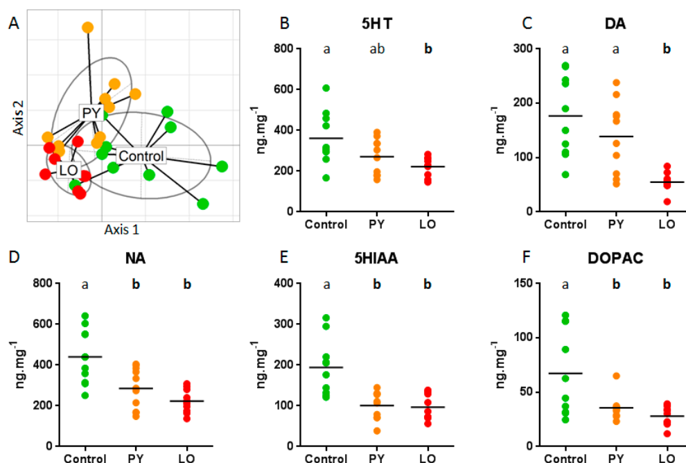
Figure 1. Analysis of monoamine brain content. (A) principal component analysis (PCA) global analysis of brain monoamine concentrations clearly identify pyrolytic (PY) and light crude oil (LO) as different from Control group. PCA axis 1 contributed to 82.1% of variability and PCA axis 2 for an additional 8.8%; (B–F) Detailed analysis of brain monoamines and metabolites concentrations in PY, LO and Control fish. Each dot represents results from an individual fish. Letters indicate significant differences at p < 0.05 between diets.
