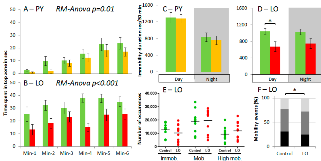
Figure 2. Analysis of behavioural traits. (A,B) Mean time spent in top zone as evaluation of anxiety using novel-tank paradigm; (C,D) Immobility duration during day and night in a 24 h-swimming test; (E) Number of events in each mobility class for individual fish and mean; and (F) Relative proportion of Immobility (black), mobility (dark grey) and high mobility (light grey) events during day period in a 24 h-swimming test. n = 12 individuals; values are mean \pm standard error of the mean; except in E (individual values and means) and F (means). In A and B since RM-Anova takes all time points into account the p -value is indicated in the figure, otherwise * indicates significant difference at p < 0.05 for PAHs diets compared to the Control.
