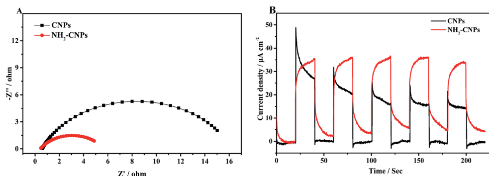
Fig. 7 (A) Nyquist plots of the CNPs (a) and \text{NH}_2 -CNPs (b). (B) The transient photocurrent responses of the CNPs (a) and \text{NH}_2 -CNPs (b) in 0.5 M \text{Na}_2\text{SO}_4 aqueous solution under visible-light ( \lambda > 420 nm) irradiation.
