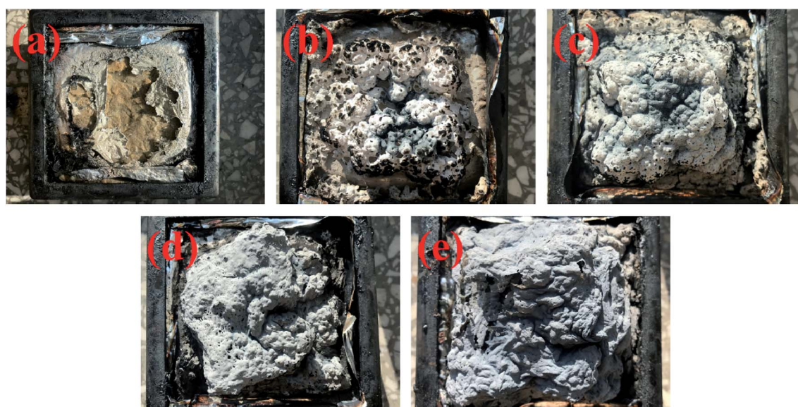
Fig. 10 Digital images of char residues from pure TPU (a), TPU/MH (b), TPU/MOF@MH (c), TPU/MH-P (d) and TPU/MOF@MH-P (e) composites after cone test.
