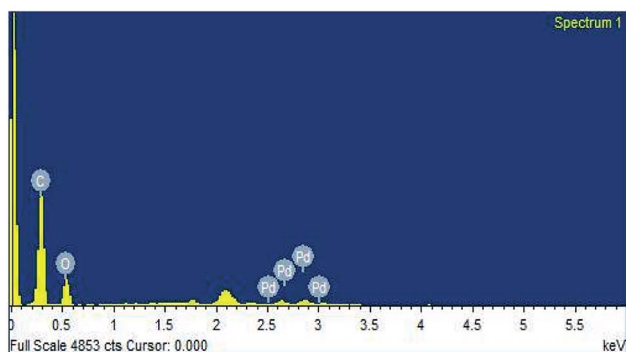
Fig. 7 The EDS spectrum of P. hysterophorus reduced PdNPs.
