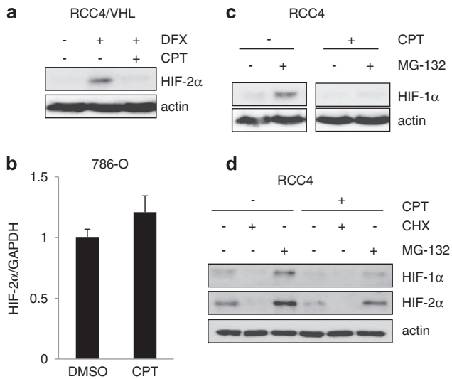
Figure 2 CPT inhibits HIF-1 \alpha and HIF-2 \alpha protein synthesis. (a) RCC4/VHL cells were incubated with 500 \mu M desferrioxamine (DFX) in the absence or presence of 2 \mu M CPT for 24 h as indicated. Whole-cell lysates were assayed by western blot for HIF-2 \alpha . Actin was used as a loading control. (b) The 786-O cells were incubated with 2 \mu M CPT or vehicle control (DMSO) for 24 h and analyzed for mRNA expression of HIF-2 \alpha by real-time quantitative PCR relative to GAPDH. (c and d) RCC4 cells were incubated with or without 2 \mu M CPT for 6 h in the absence or presence of 10 \mu M MG-132 or 10 \mu M cycloheximide (CHX) for the final 3 h as indicated. Whole-cell lysates were assayed by western blot for HIF-1 \alpha and HIF-2 \alpha . Actin was used as a loading control
