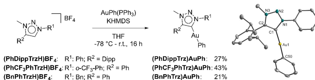
Scheme 5. Synthesis of the phenyl triazolone gold complexes and molecular structure of (PhDippTrz)AuPh in the crystal. Thermal ellipsoids are drawn at the 50% probability level. Hydrogen atoms are omitted for clarity.
