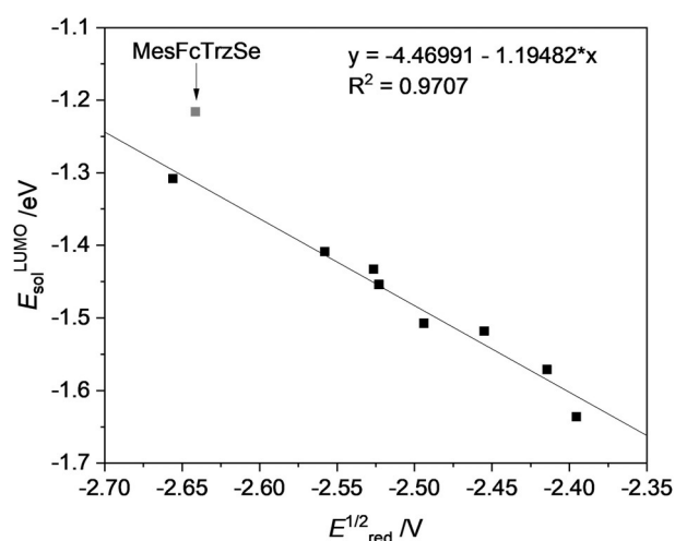
Figure 6. Correlation of E_{\text{sol}}^{\text{LUMO}} and E^{1/2}_{\text{red}} ( \cong E^{\circ}_{\text{red}} ) with a goodness-of-fit R^2 = 0.97 . MesFcTrzSe was treated as an outlier and is not included in the correlation calculations.
