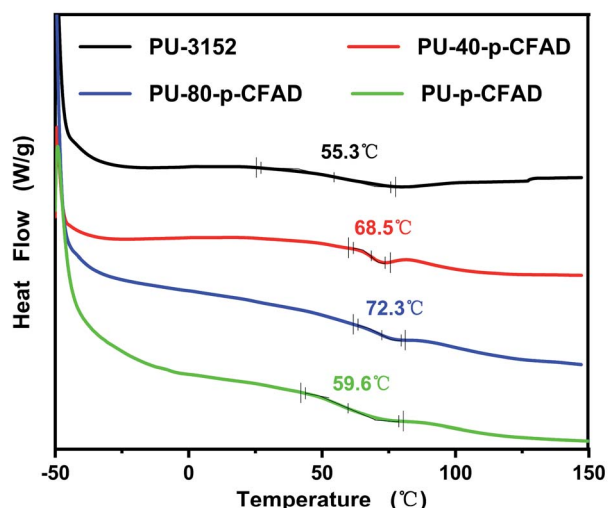
Fig. 7 DSC plot lines and thermal transition of PU foams.
