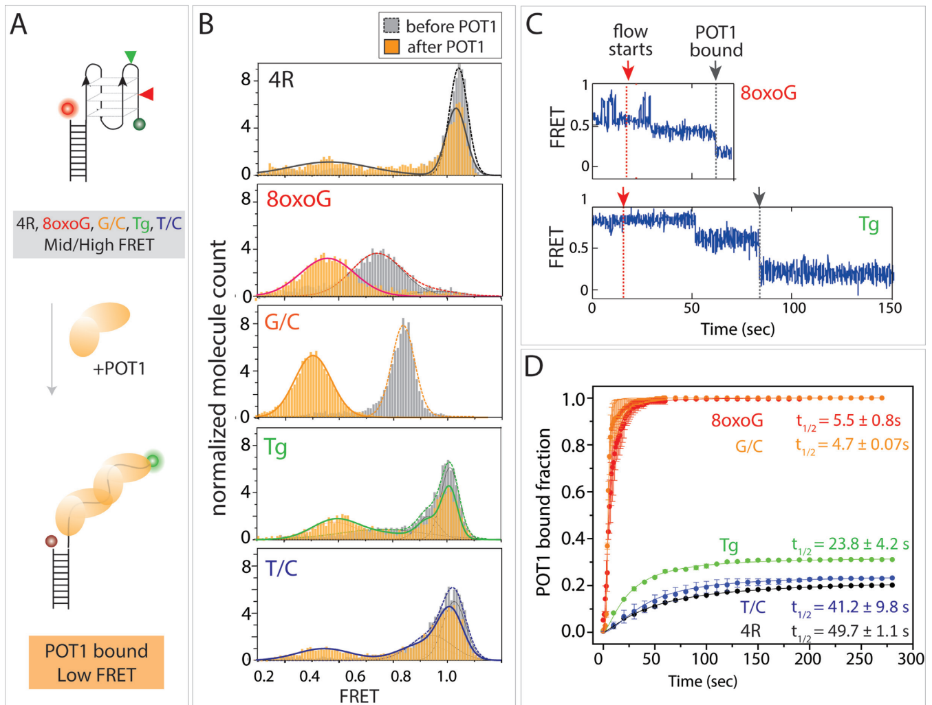
Figure 4. POT1 binding to telomeric G4 is enhanced by 8oxoG, but not significantly by Tg. (A) Study design for testing telomeric G4 accessibility to POT1 protein (100 nM). High FRET is expected to convert to low FRET upon POT1 association. (B) FRET histogram before (gray) and after (orange) POT1 addition. (C) Single molecule traces displaying the moment of C4 flow and FRET decrease due to POT1 binding. (D) Kinetic analysis of POT1 binding for all the DNA constructs tested. Error bars represent the standard deviation between trials.
